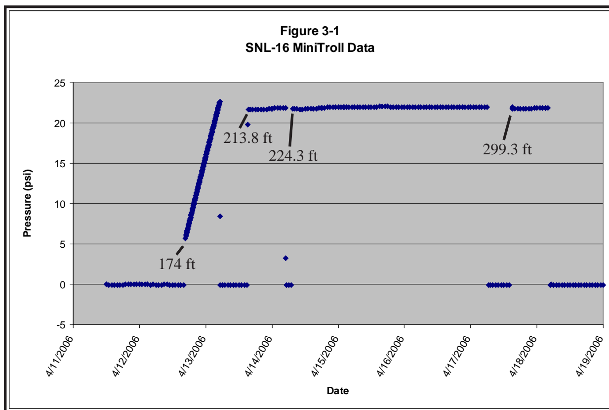
Figure 3-1. Plot of pressures measured by miniTroll in SNL-16 during drilling and coring period. MiniTroll was allowed to run continuously and was placed at a depth of 170 ft each recording period. Bottom of hole is shown at the beginning of each recording period.
