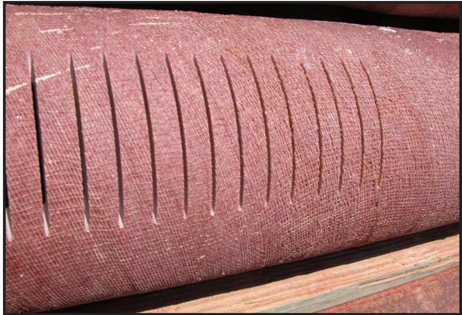
Figure 3-2. Screen used in SNL-16 with 0.070-inch slots. Photo by Dennis W. Powers.
